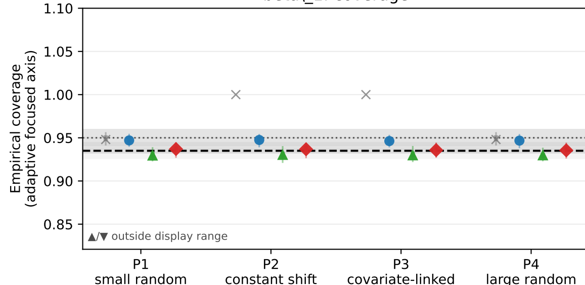
beta\_1: coverage
