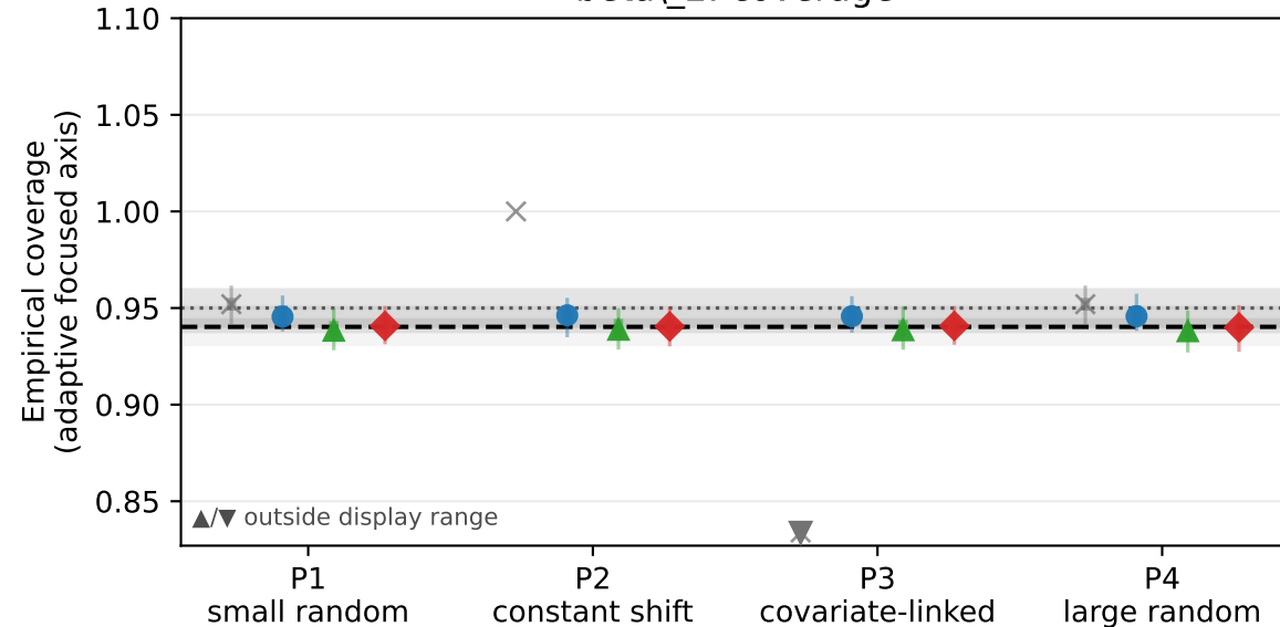
beta\_2: coverage
