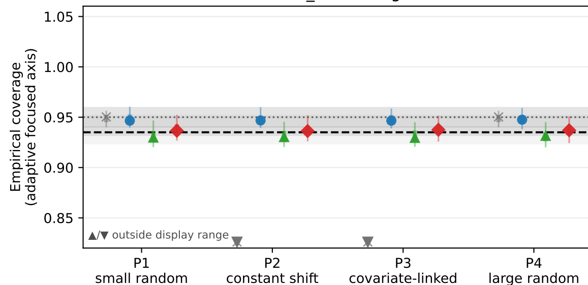
beta\_0: coverage
