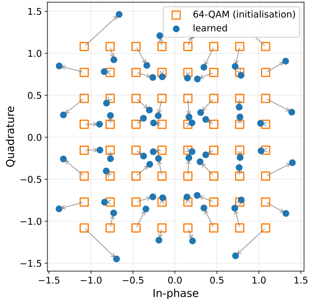
Where the gain comes from: point displacement
