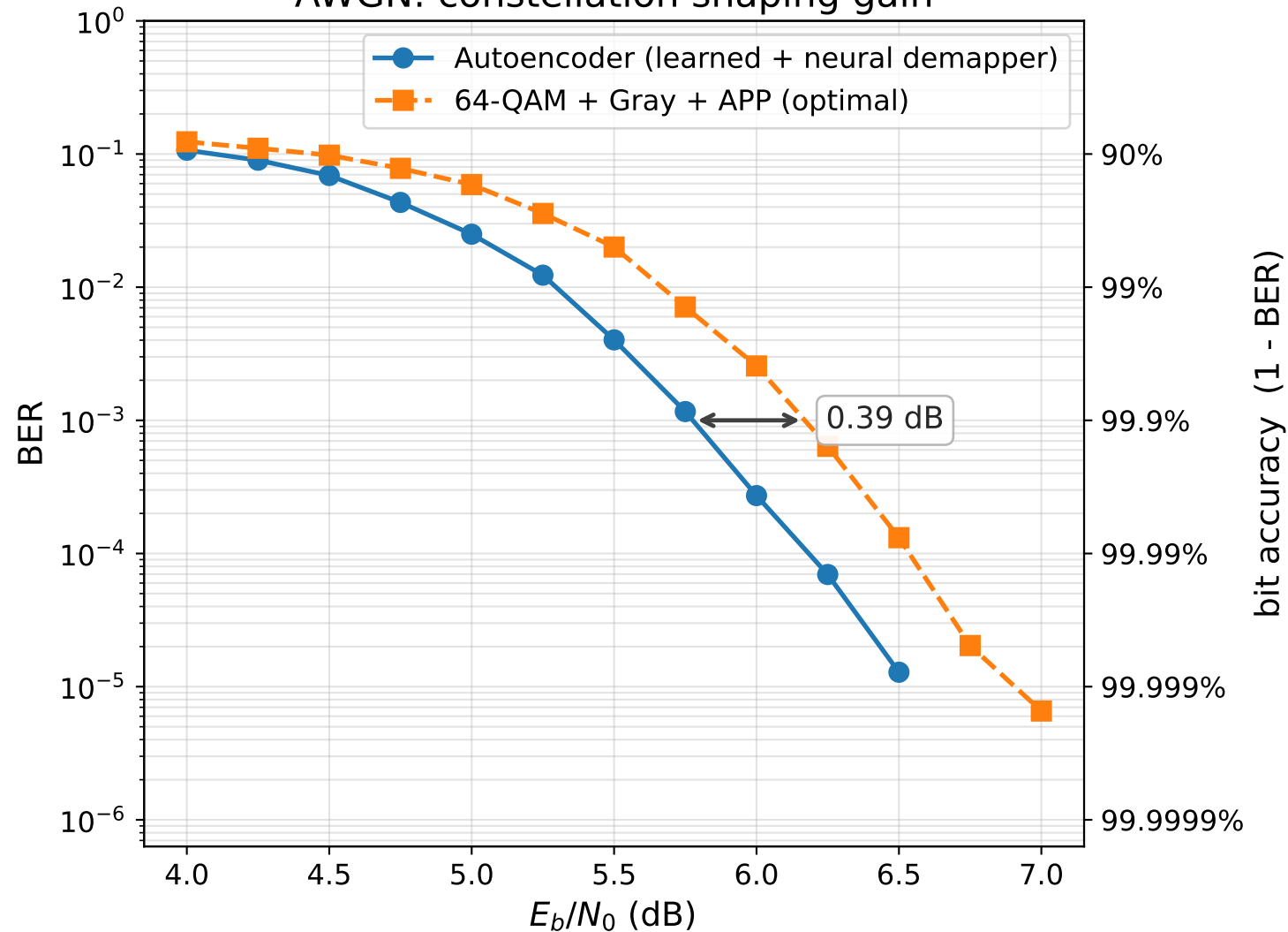
AWGN: constellation shaping gain
