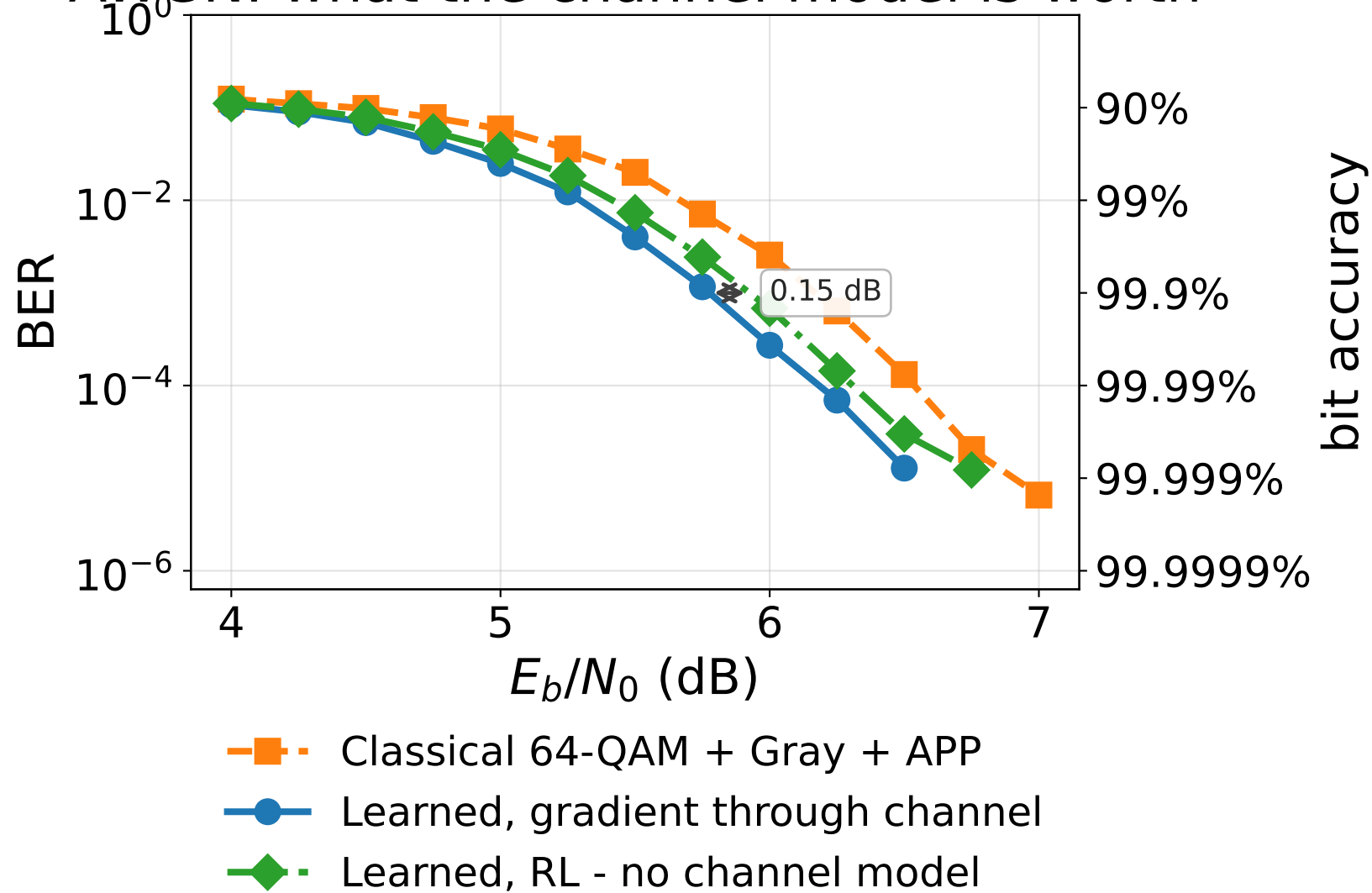
AWGN: what the channel model is worth
