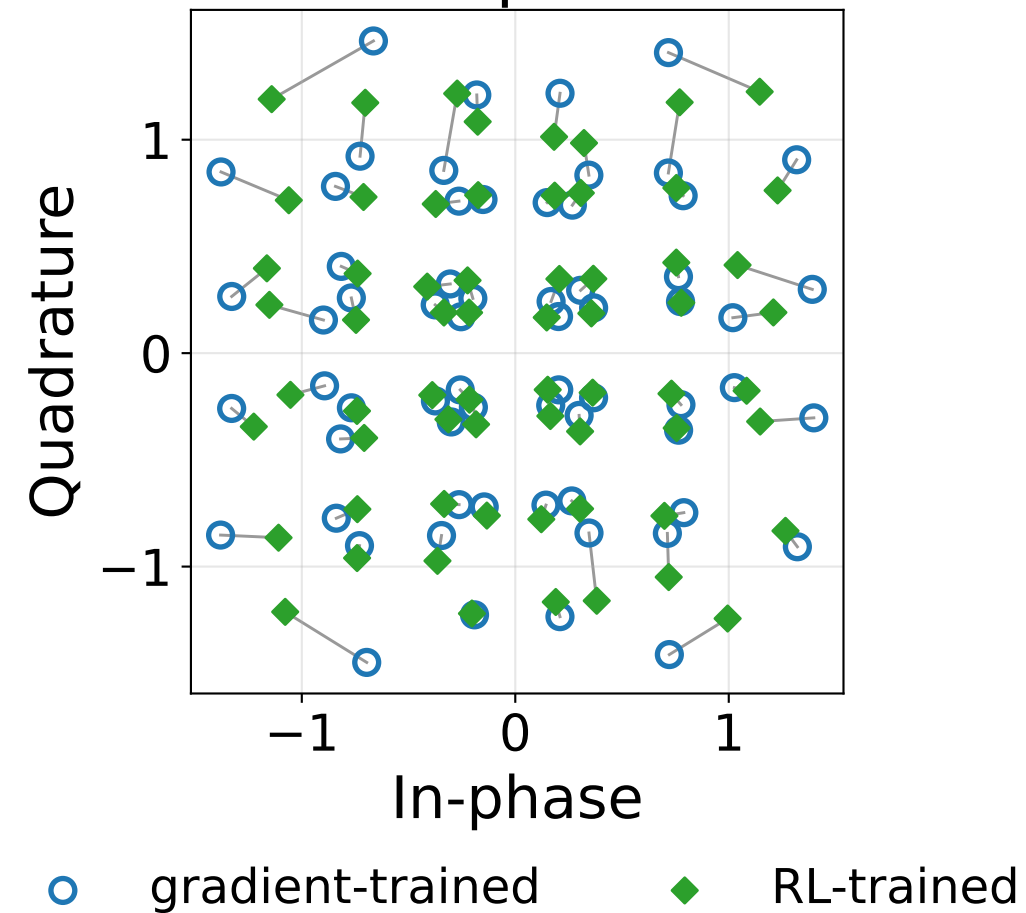
Where each method puts the same symbol
