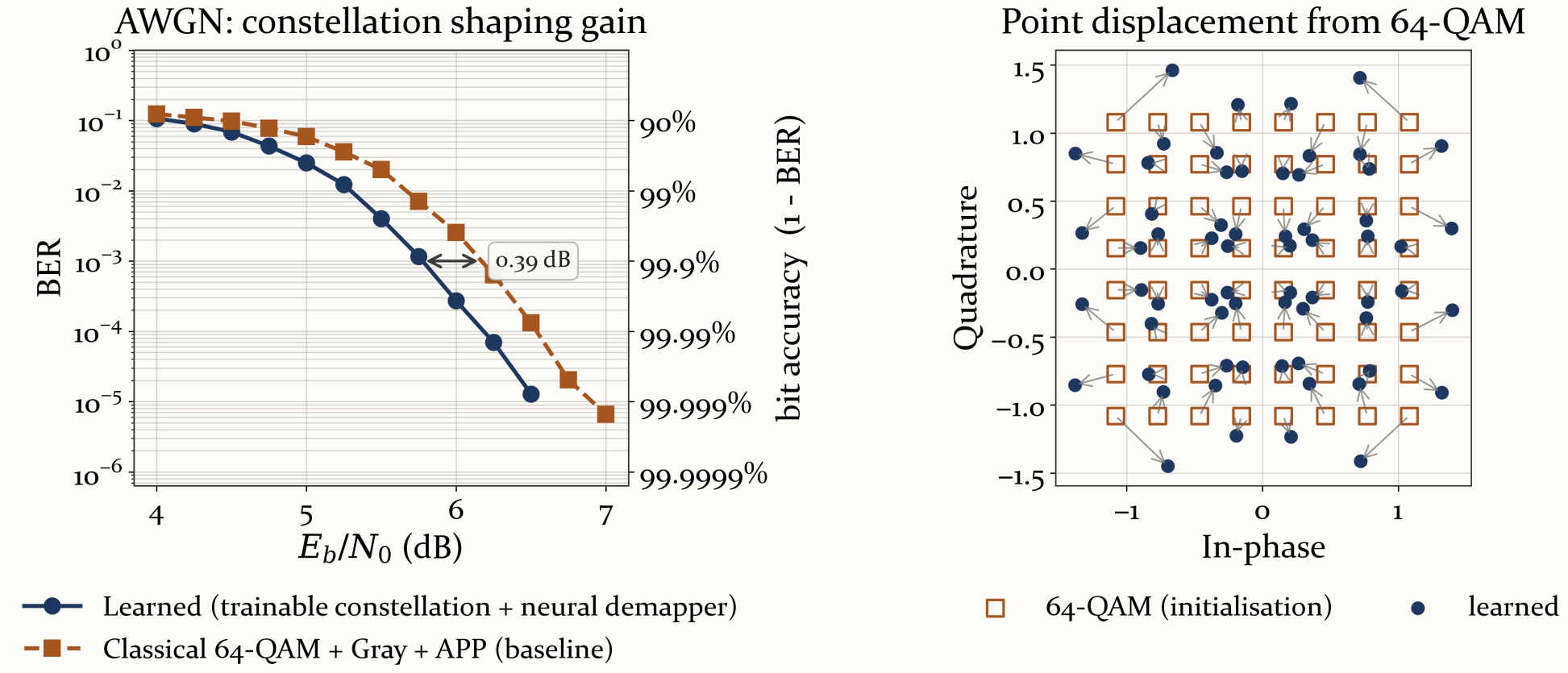
Fig. 2 — The learned system against 64-QAM with Gray labelling and APP demapping, on identical channel realisations.
