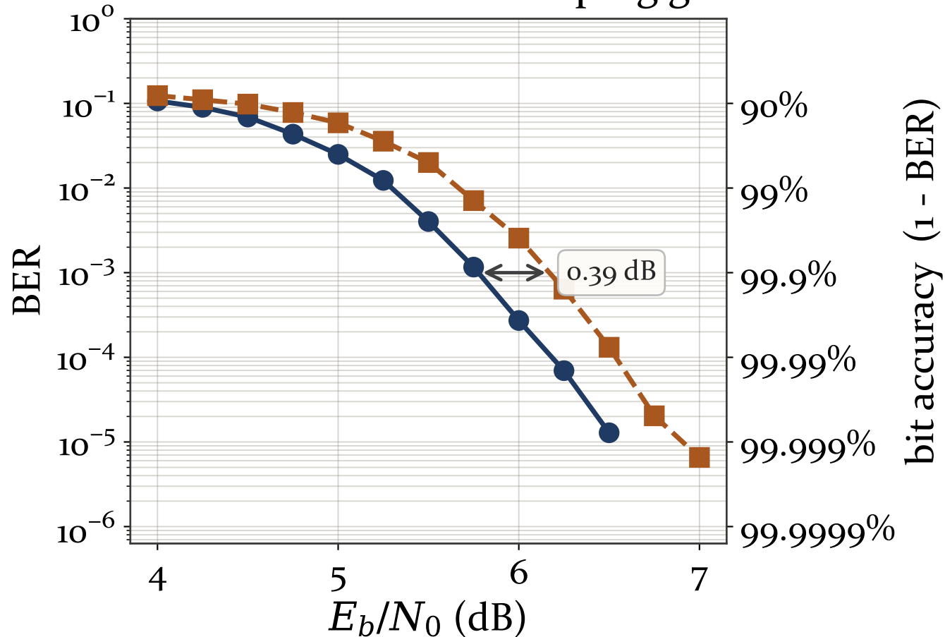
AWGN: constellation shaping gain
