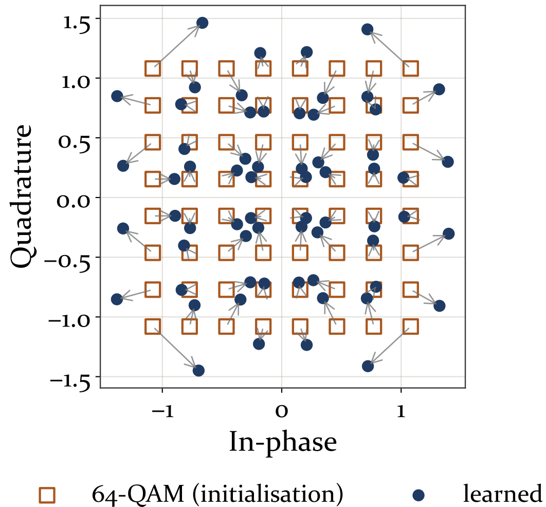
Point displacement from 64-QAM
