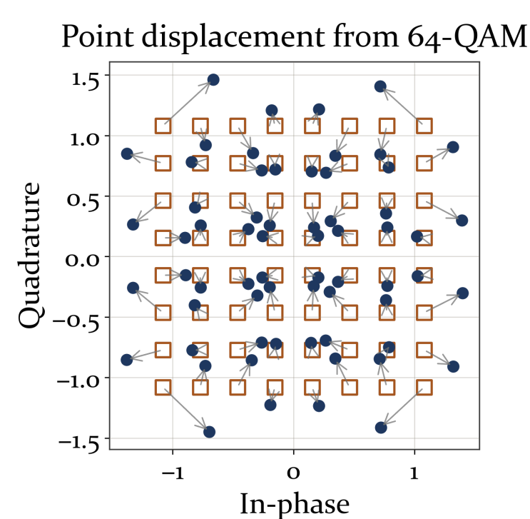
□ 64-QAM (initialisation) ● learned
