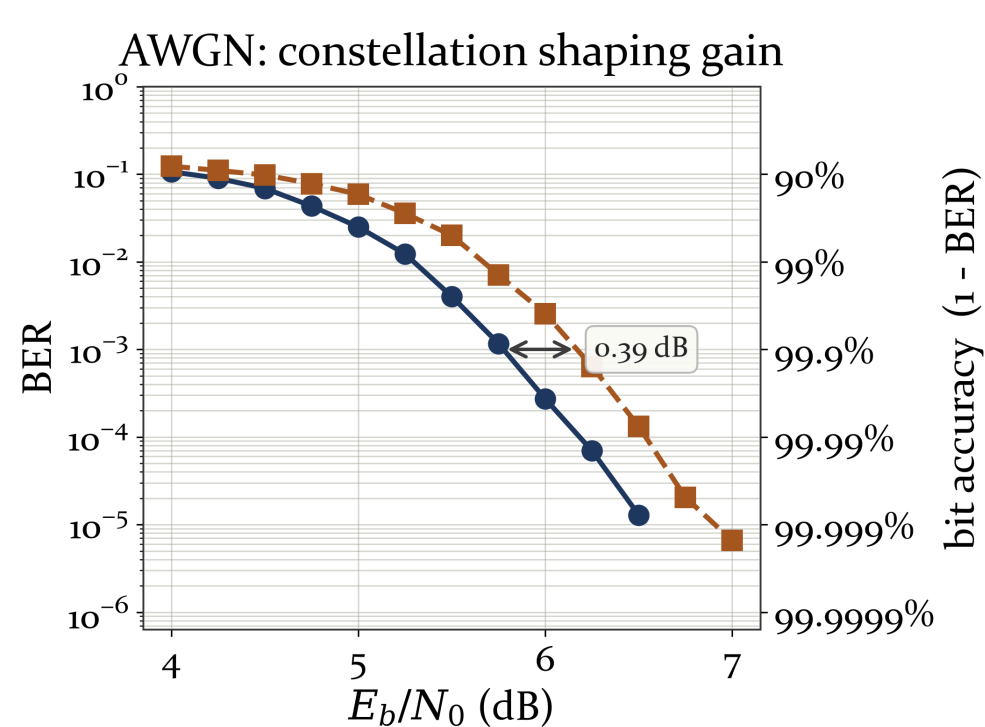
— Learned (trainable constellation + neural demapper) — Classical 64-QAM + Gray + APP (baseline)
