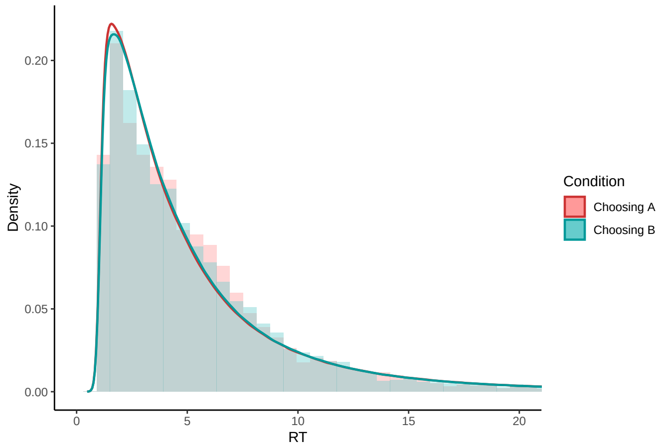
Empirical vs. Predicted RT Distributions (cpt_ccss_7o / n_a_s)
