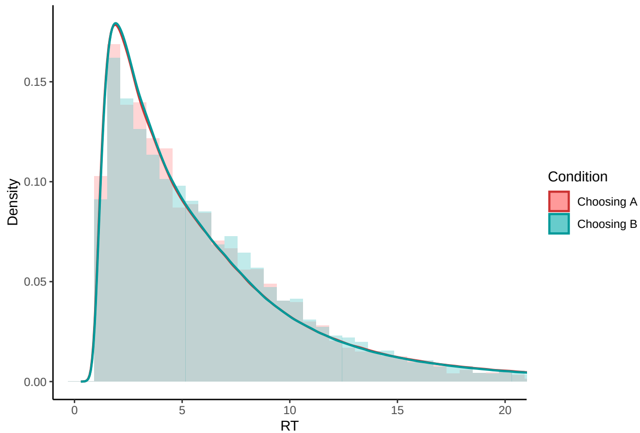
Empirical vs. Predicted RT Distributions (cpt_ccss / n_a_s)
