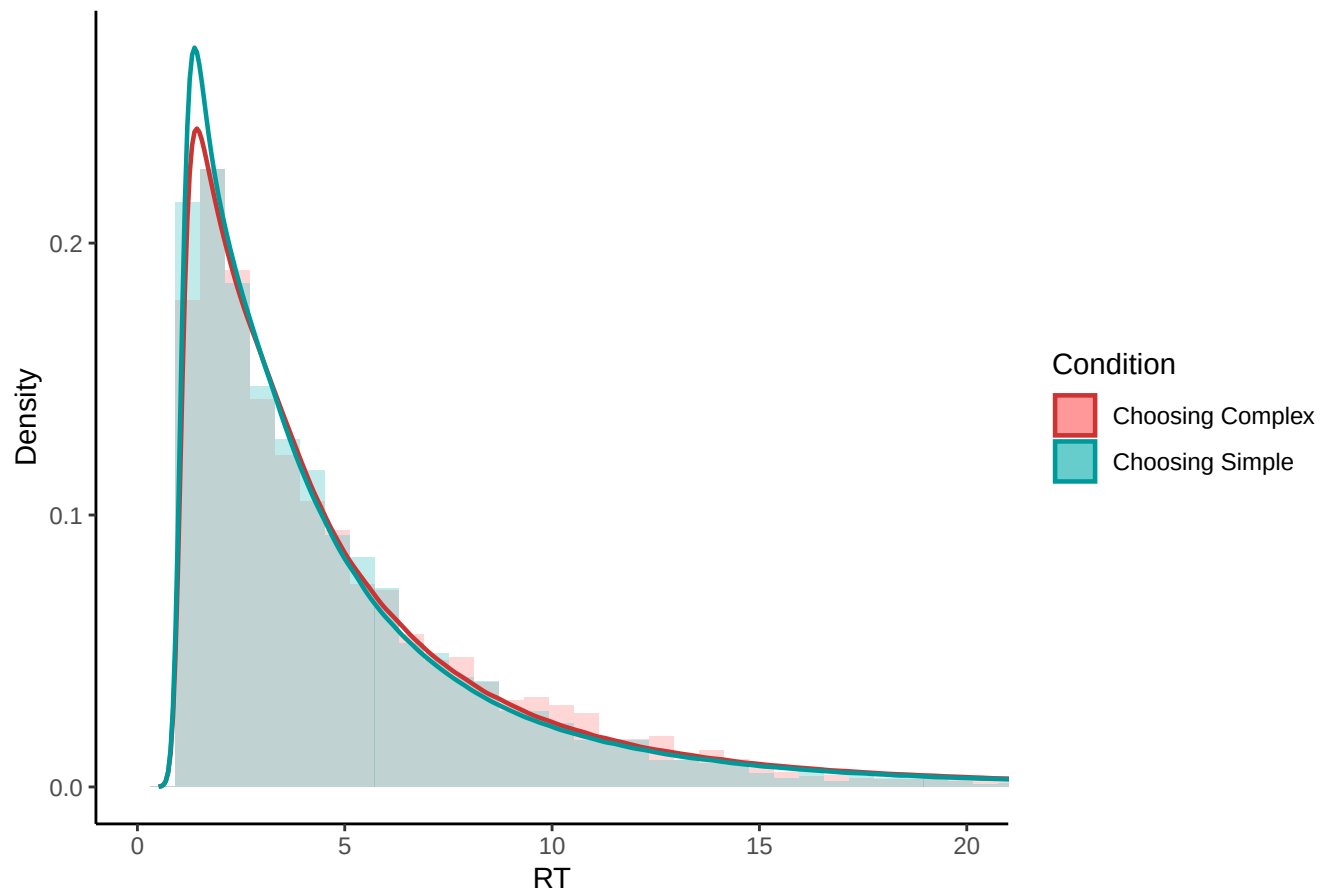
Empirical vs. Predicted RT Distributions (cpt_cs_7o / sp_dr)
