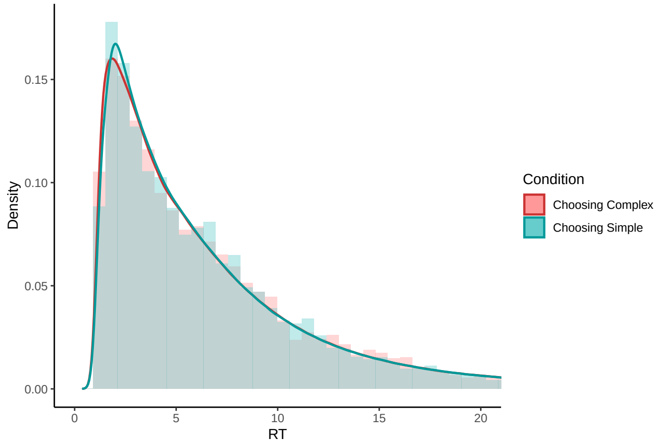
Empirical vs. Predicted RT Distributions (cpt_cs / sp_dr)
