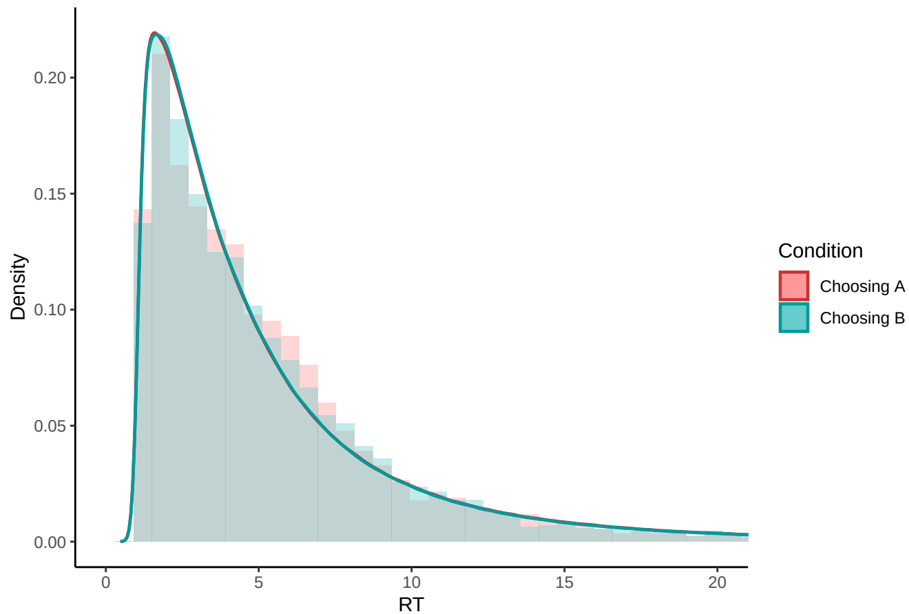
Empirical vs. Predicted RT Distributions (mv_ccss / n_r_a_s)
