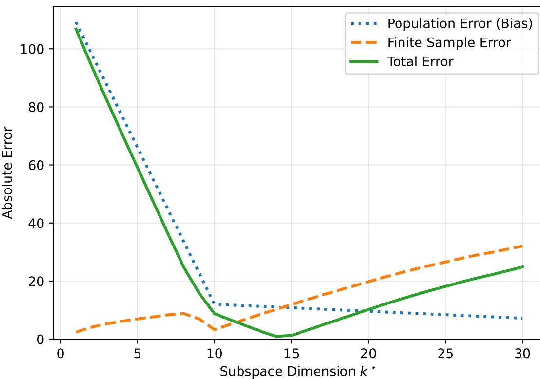
WPP Trade-off ( \alpha = 0.0 )
