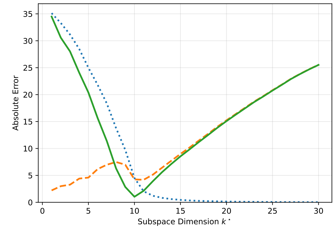
LB Trade-off ( \alpha = 1.5 )
