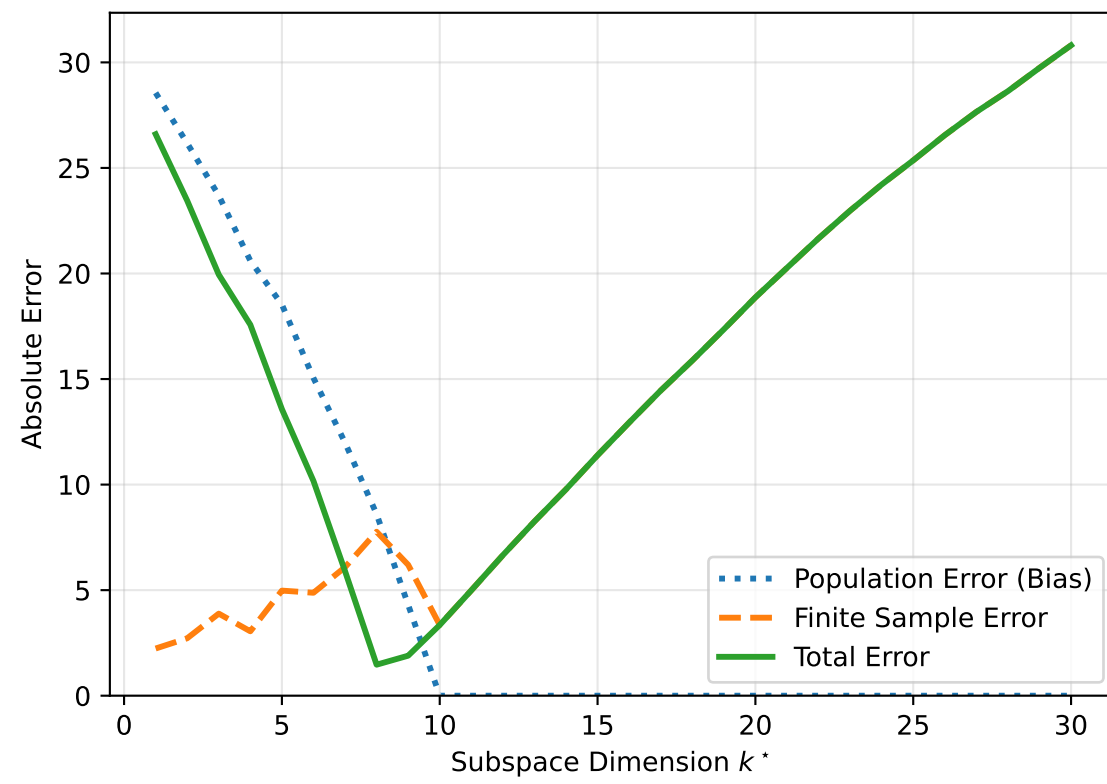
LB Trade-off ( \alpha = 0.0 )
