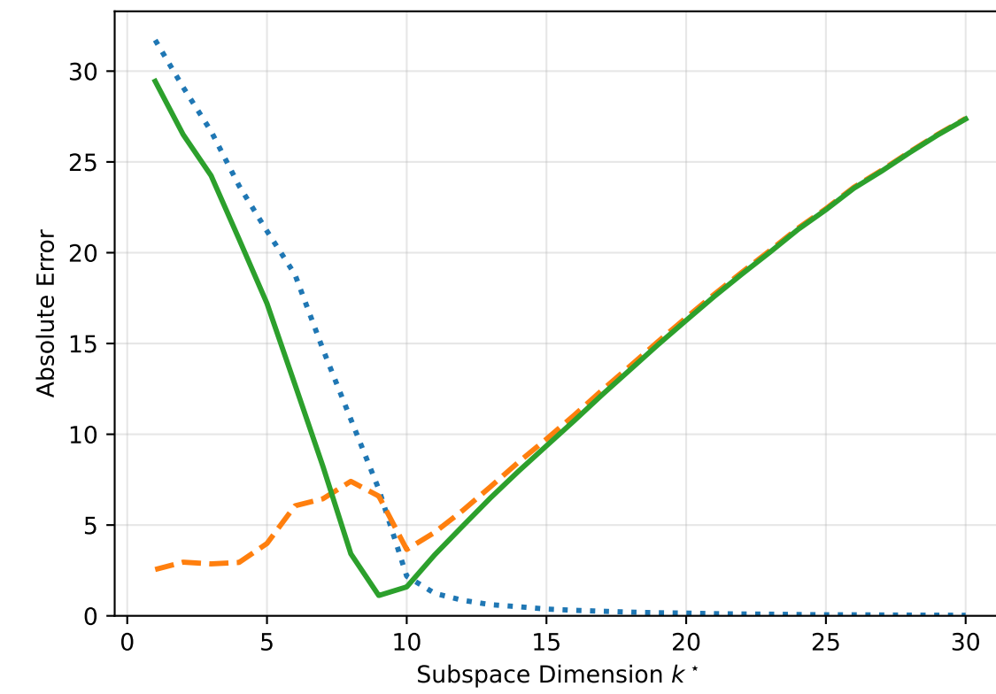
LB Trade-off ( \alpha = 1.0 )
