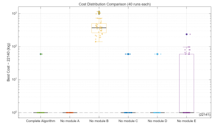
(c) kroB100
