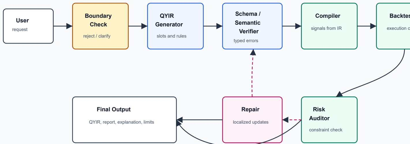
Figure 2. QSGA Architecture
