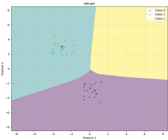
Unlearned
