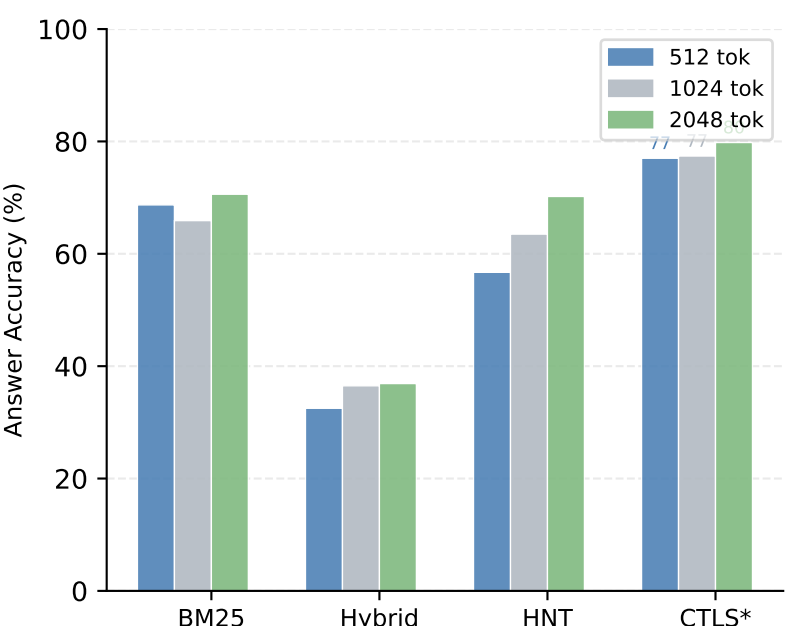
Selector Comparison across Token Budgets
