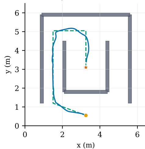
(f) Serpentine 1297 steps | min clearance 0.19 m
