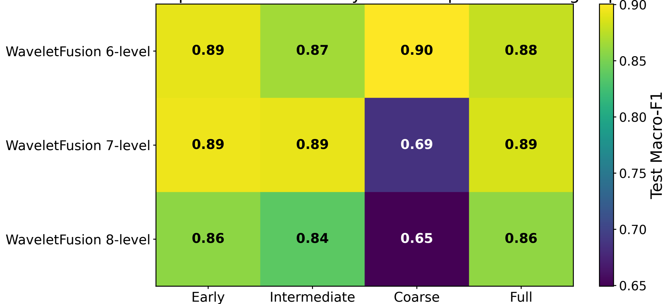
Heatmap of Test Macro-F1 by model depth and scale group
