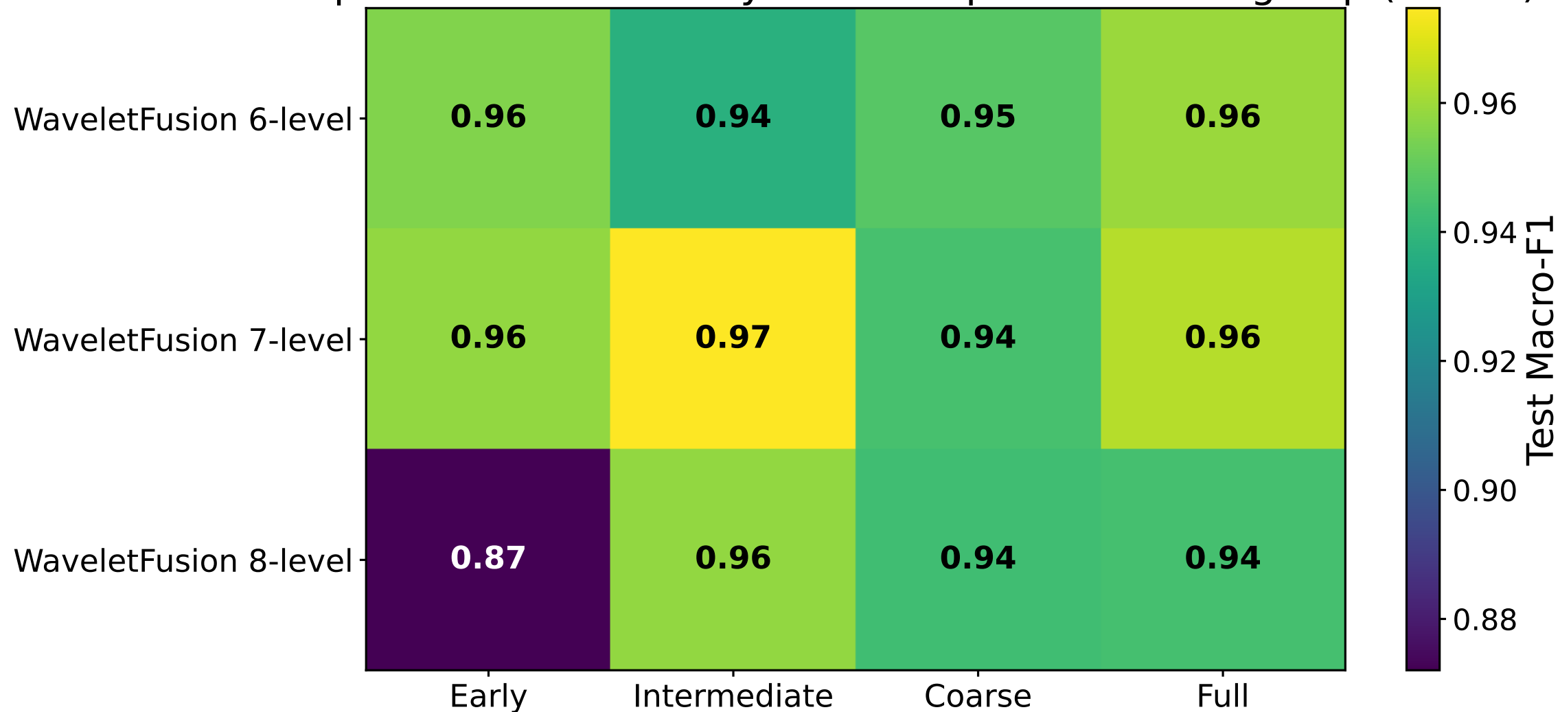
Heatmap of Test Macro-F1 by model depth and scale group (Br35H)
