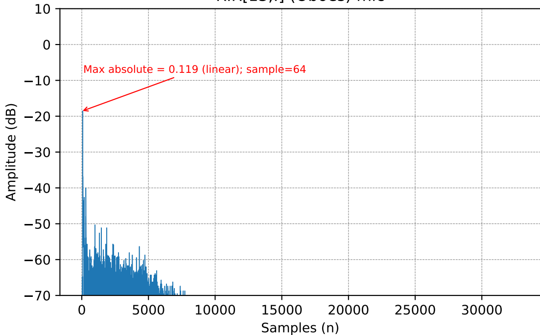
RIR[13,:] (Oboes) mic
