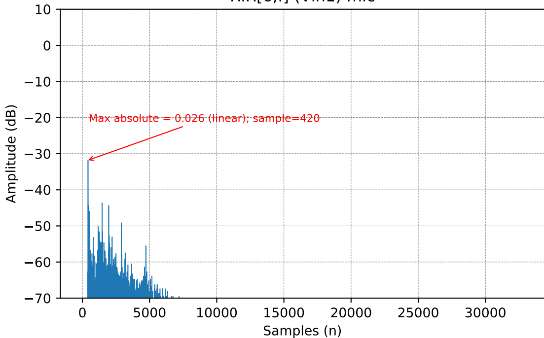
RIR[6,:] (Vln1) mic
