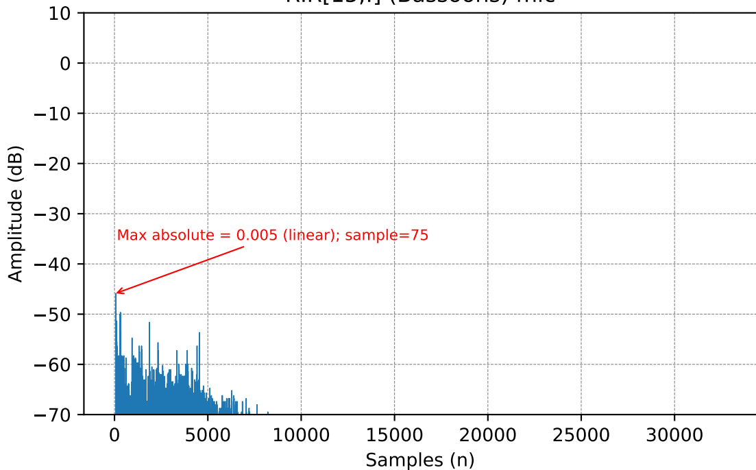
RIR[15,:] (Bassoons) mic
