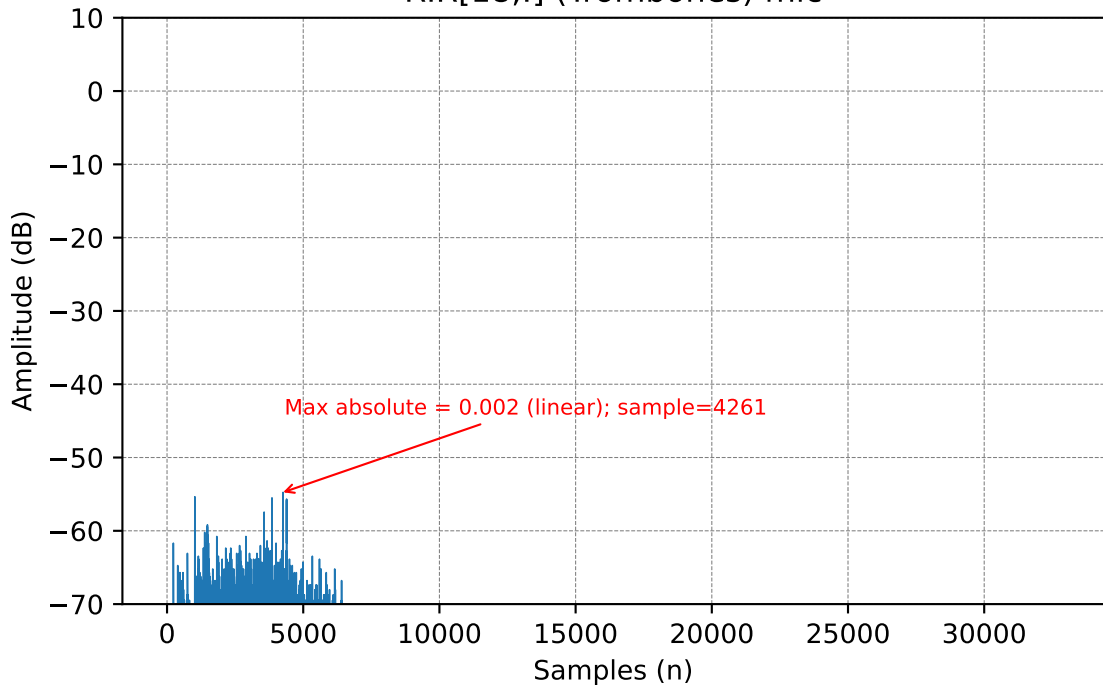
RIR[18,:] (Trombones) mic
