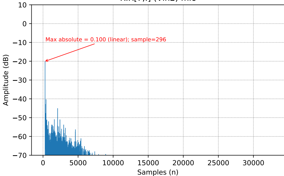
RIR[7,:] (Vln2) mic
