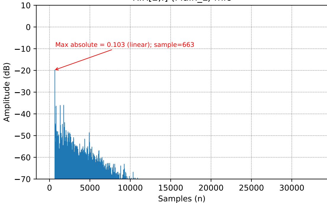
RIR[2,:] (Main_L) mic
