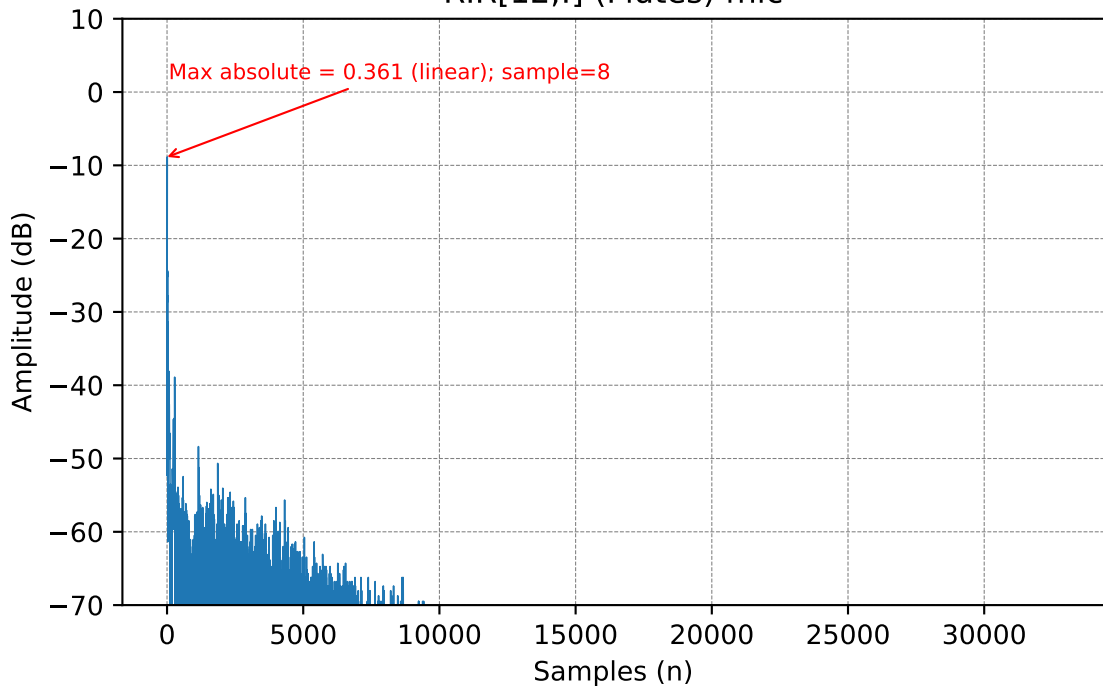
RIR[12,:] (Flutes) mic
