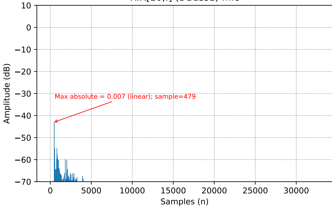
RIR[10,:] (DBass1) mic
