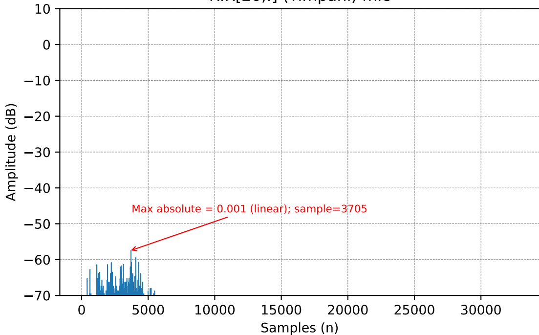
RIR[20,:] (Timpani) mic
