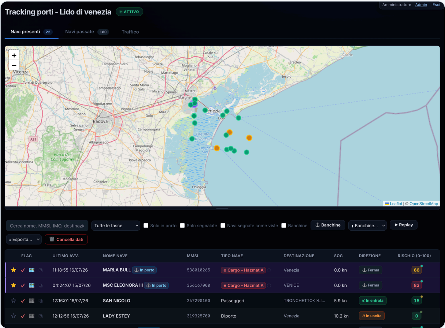
Current ships tab: map with markers colored by risk and detailed table below.
