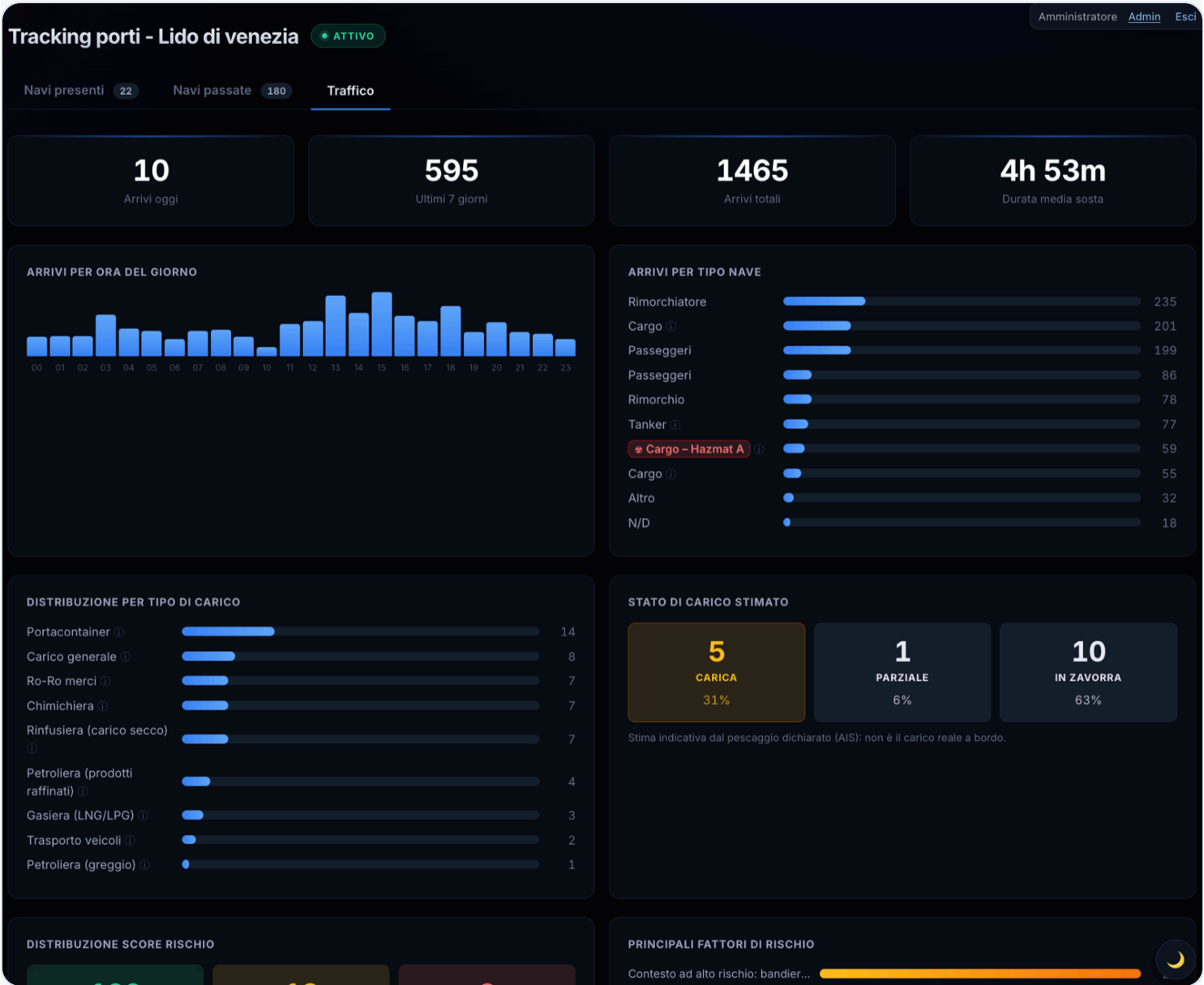
Traffic tab: stat tiles at the top, and charts for arrivals by hour, ship type, risk distribution, and daily trend.
