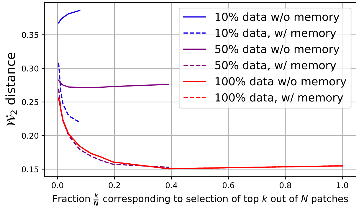
\mathcal{W}_2 distance vs k (1024 synthesis vs 256 examples)
