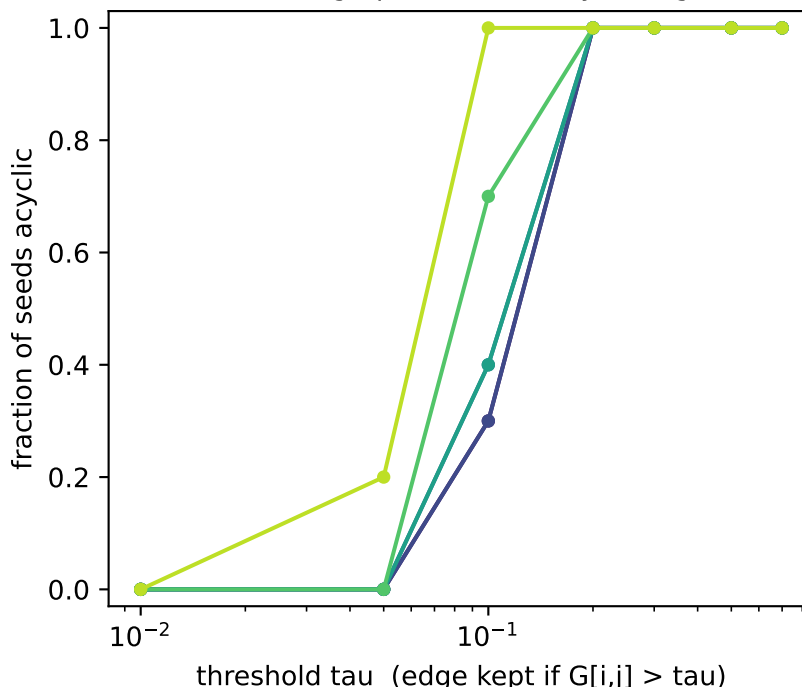
H. Binarised graph is a DAG only at large tau
