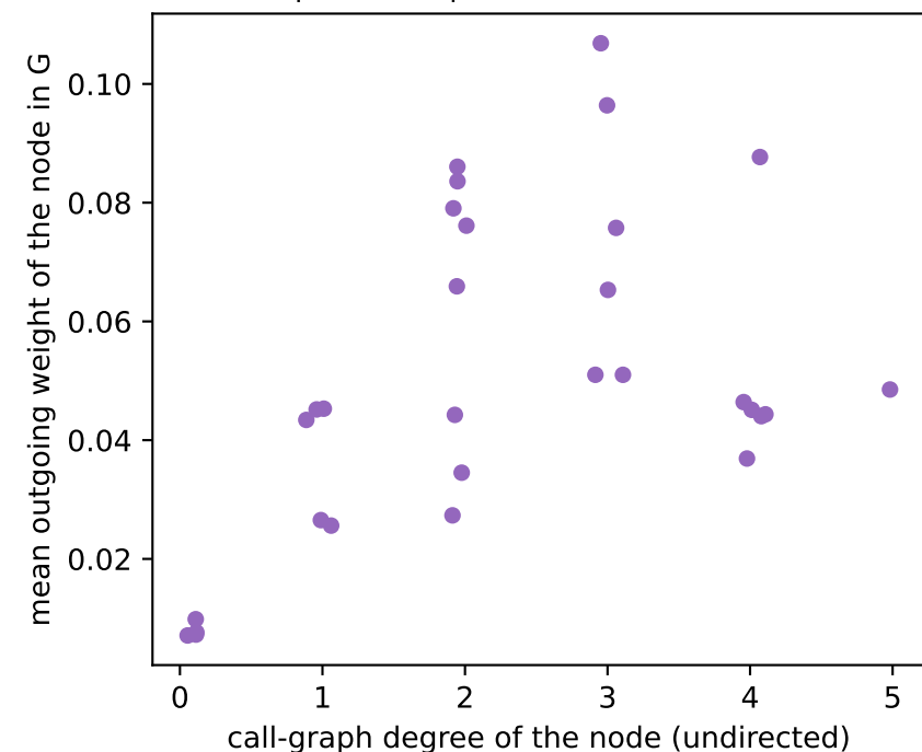
C. Node-level view (exploratory) per-seed Spearman 0.45 +/- 0.11
