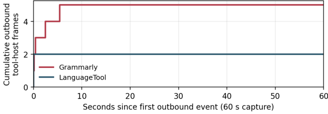
Fig. 3: Outbound traffic to the tool’s own host is a single burst at the moment of paste, then silence for the rest of the 60 s capture. Cumulative client-to-server frames to grammarly.com and languagetool.org , one representative run each.
