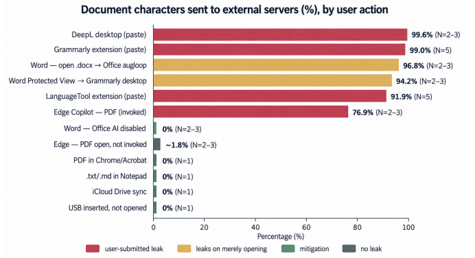
Fig. 4: Document characters transmitted to external servers, by user action. Submitting to a cloud AI tool or simply opening the document in Word transmits nearly all of it and every planted secret; one Office setting drops the Word transmission to 0%, and passive receipt or non-AI viewers transmit nothing. Colour encodes the interaction class; the per-bar run count N varies (see Table III), so equal bar lengths are not equal statistical weight.
