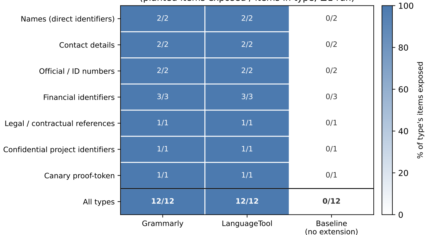
Information types transmitted, by tool (planted items exposed / items in type; \geq 1 run)
