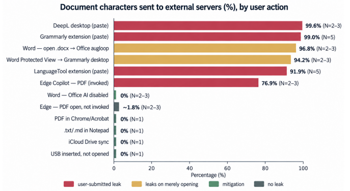
Fig. 8: Document characters transmitted to external servers, by user action. Submitting to a cloud AI tool (DeepL, Grammarly, LanguageTool, invoked Edge Copilot) or merely opening the document in Microsoft Word leaks nearly all of it and every planted secret; disabling one Office setting drops the Word leak to 0%, and passive receipt (USB, iCloud sync) or non-AI viewers (Notepad, Acrobat, browser PDF) transmit no document content. Colour encodes the interaction class; N is the number of independent runs (browser writing assistants 5, standard deviation 0; Word/DeepL/Edge-Copilot 2–3; other host probes single-run), so equal bar lengths should not be read as equal statistical weight.
