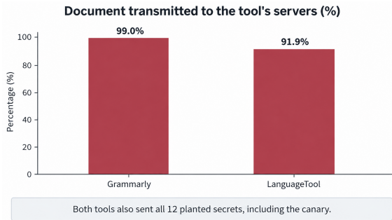
Fig. 5: Share of the confidential document transmitted to each tool’s servers by default. Both grammar checkers transmit essentially the whole document and all twelve planted secrets (the no-extension baseline, in Table II, transmits nothing).
