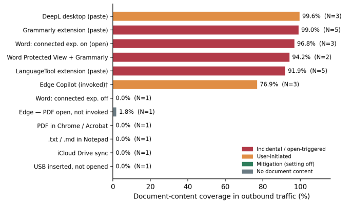
Fig. 3: Document-content coverage in outbound traffic, by user action and surface. Colour encodes the interaction class (incidental/open-triggered, user-initiated, the connected-experiences-off mitigation, and no document content). Exact run counts N are shown per bar; single-run rows are individual observations, not repeatability estimates. Edge/Copilot (†) is a lower bound because some of its channels were certificate-pinned.
