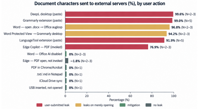
Fig. 3: Document characters transmitted to external servers, by user action. Submitting to a cloud AI tool or simply opening the document in Word leaks nearly all of it and every planted secret; one Office setting drops the Word leak to 0%, and passive receipt or non-AI viewers transmit nothing. Colour encodes the interaction class; the per-bar run count N varies (see Table III), so equal bar lengths are not equal statistical weight.
