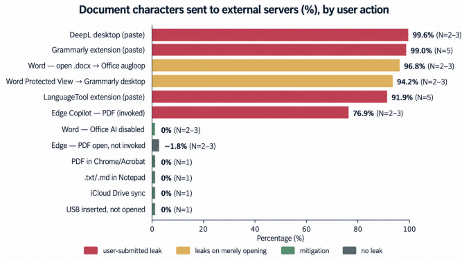
Fig. 6: Document characters transmitted to external servers, by user action. Submitting to a cloud AI tool (DeepL, Grammarly, LanguageTool, invoked Edge Copilot) or merely opening the document in Microsoft Word leaks nearly all of it and every planted secret; disabling one Office setting drops the Word leak to 0%, and passive receipt (USB, iCloud sync) or non-AI viewers (Notepad, Acrobat, browser PDF) transmit no document content. Colour encodes the interaction class; N is the number of independent runs (browser writing assistants 5, standard deviation 0; Word/DeepL/Edge-Copilot 2–3; other host probes single-run), so equal bar lengths should not be read as equal statistical weight.
