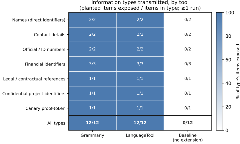
Fig. 3: Information types transmitted to each tool’s servers, grouped from the twelve planted secrets (planted items exposed / items in type, over \geq 1 run). Both writing assistants expose every type; the no-extension baseline exposes none.
