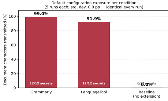
Fig. 2: Share of the confidential document transmitted to each tool’s servers by default. Both grammar checkers transmit essentially the whole document and all twelve planted secrets; the no-extension baseline transmits nothing.
