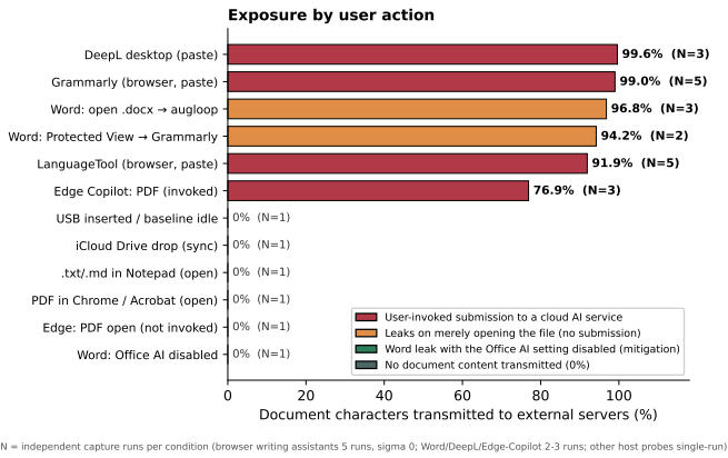
Fig. 5: Document characters transmitted to external servers, by user action. Submitting to a cloud AI tool (DeepL, Grammarly, LanguageTool, invoked Edge Copilot) or merely opening the document in Microsoft Word leaks nearly all of it and every planted secret; disabling one Office setting drops the Word leak to 0%, and passive receipt (USB, iCloud sync) or non-AI viewers (Notepad, Acrobat, browser PDF) transmit no document content. Colour encodes the interaction class; N is the number of independent runs (browser writing assistants 5, standard deviation 0; Word/DeepL/Edge-Copilot 2–3; other host probes single-run), so equal bar lengths should not be read as equal statistical weight.
