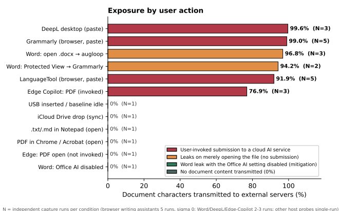
Fig. 8: Document characters transmitted to external servers, by user action. Submitting to a cloud AI tool (DeepL, Grammarly, LanguageTool, invoked Edge Copilot) or merely opening the document in Microsoft Word leaks nearly all of it and every planted secret; disabling one Office setting drops the Word leak to 0%, and passive receipt (USB, iCloud sync) or non-AI viewers (Notepad, Acrobat, browser PDF) transmit no document content. Colour encodes the interaction class; N is the number of independent runs (browser writing assistants 5, standard deviation 0; Word/DeepL/Edge-Copilot 2–3; other host probes single-run), so equal bar lengths should not be read as equal statistical weight.
