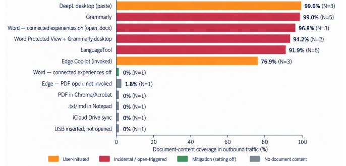
Fig. 3: Document-content coverage in outbound traffic, by user action and surface. Colour encodes the interaction class (incidental/open-triggered, user-initiated, the connected-experiences-off mitigation, and no document content). Exact run counts N are shown per bar; single-run rows are individual observations, not repeatability estimates. Edge/Copilot is a lower bound because some of its channels were certificate-pinned.
