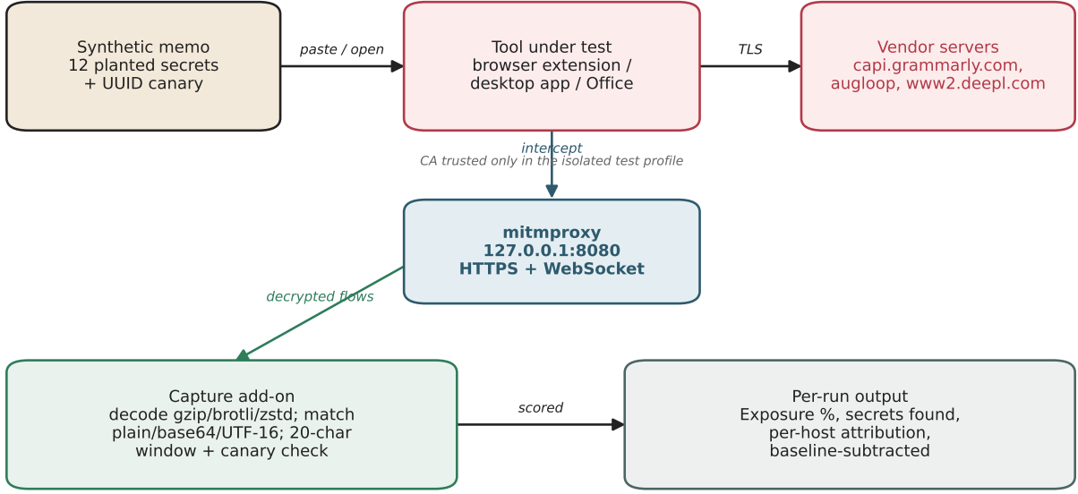
Fig. 1: Overview of the measurement pipeline. The synthetic memo (with twelve planted secrets and a UUID canary) enters the tool under test, whose traffic is intercepted by mitmproxy on 127.0.0.1:8080; a capture add-on decodes and matches the outbound flows to produce a baseline-subtracted exposure figure and per-host attribution.
