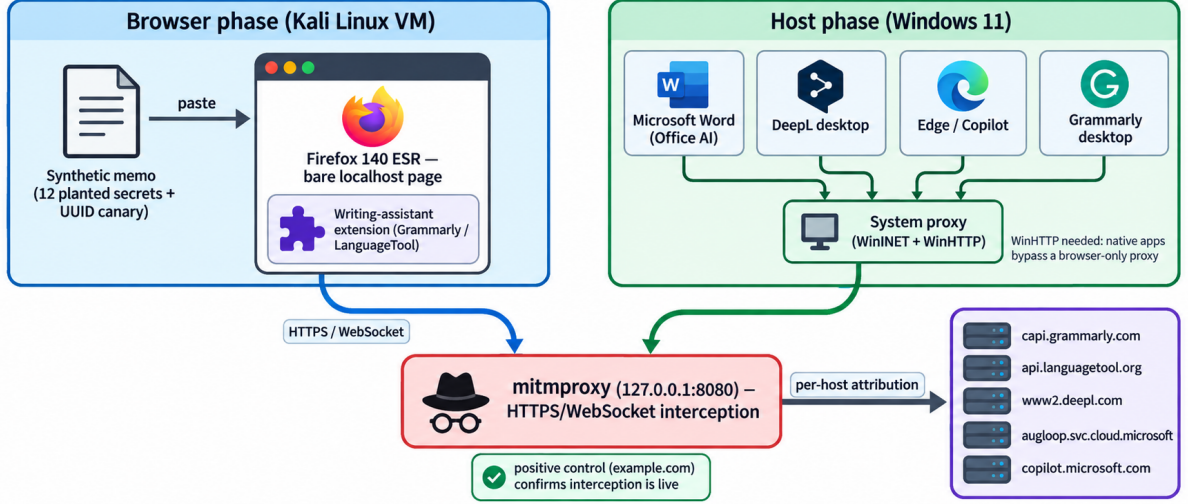
Fig. 1: Experimental setup. In the browser phase (isolated Kali Linux VM), the synthetic memo is pasted into a bare local page and read by the writing-assistant extension. In the host phase (Windows 11), native applications and Office reach the network through the system proxy (WinINET + WinHTTP, the latter required because native clients bypass a browser-only proxy). Both phases route through mitmproxy (127.0.0.1:8080); a positive control (example.com) confirms interception is live, and every flow is attributed to its destination host.
