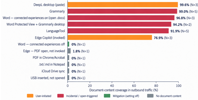
Fig. 3: Document-content coverage in outbound traffic, by user action and surface. Exact run counts N are shown per bar; single-run rows are individual observations, not repeatability estimates. Edge/Copilot is a lower bound (some channels were certificate-pinned). The “no document content” class means no attributable document-specific content: the passive Edge bar’s 1.8% is a generic boilerplate phrase, not a planted secret.
