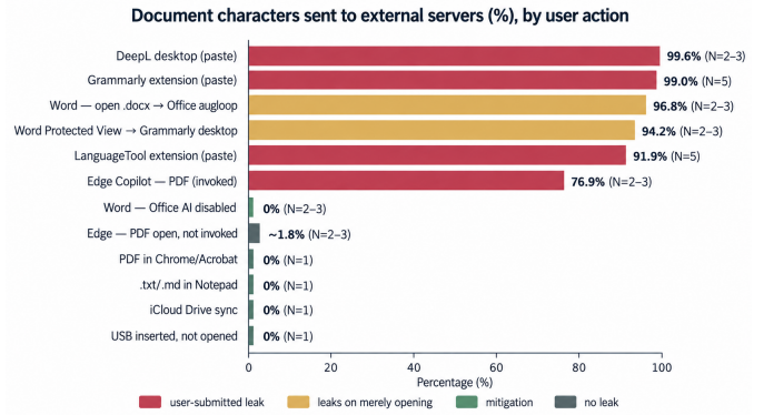
Fig. 5: Document characters transmitted to external servers, by user action. Submitting to a cloud AI tool (DeepL, Grammarly, LanguageTool, invoked Edge Copilot) or simply opening the document in Microsoft Word leaks nearly all of it and every planted secret; disabling one Office setting drops the Word leak to 0%, and passive receipt (USB, iCloud sync) or non-AI viewers (Notepad, Acrobat, browser PDF) transmit no document content. Colour encodes the interaction class; N is the number of independent runs (browser writing assistants 5, standard deviation 0; Word/DeepL/Edge-Copilot 2–3; other host probes single-run), so equal bar lengths should not be read as equal statistical weight.
