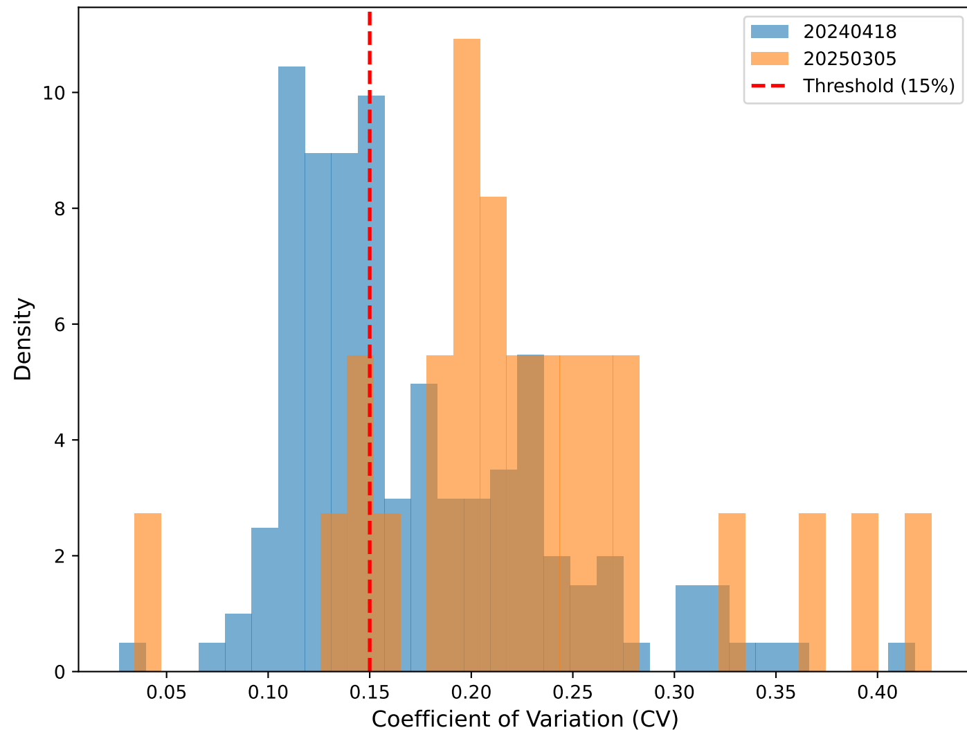
CV Distribution
