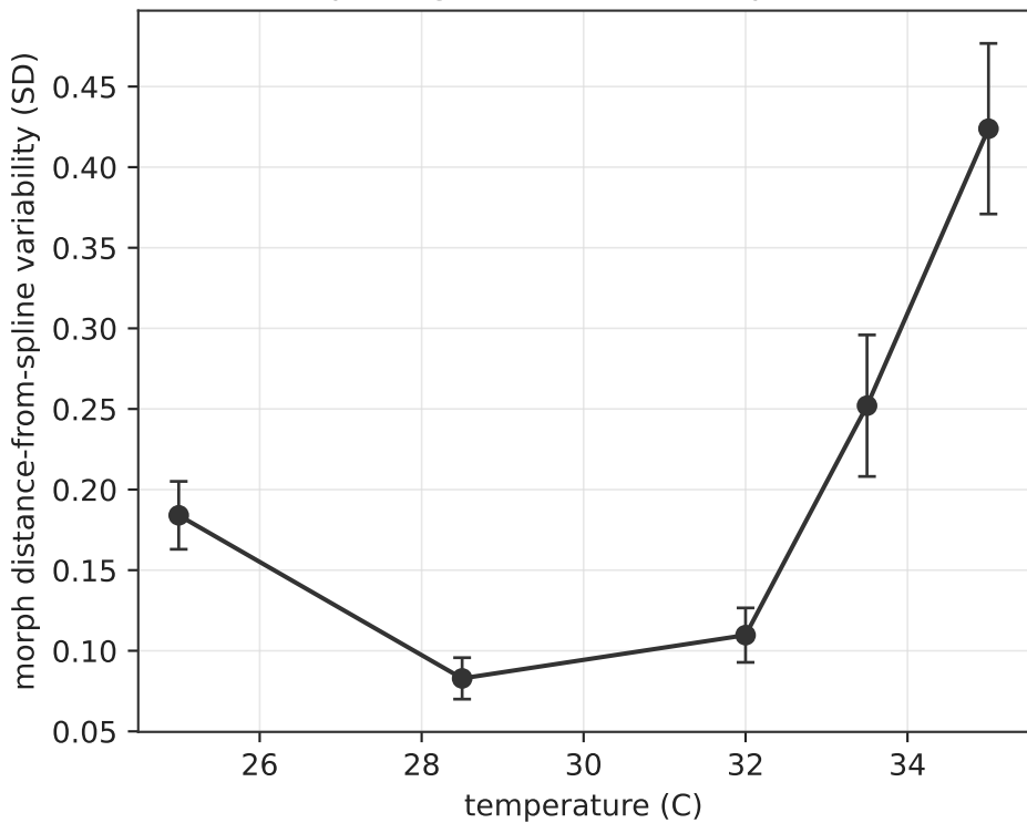
Morphological noise vs temperature
