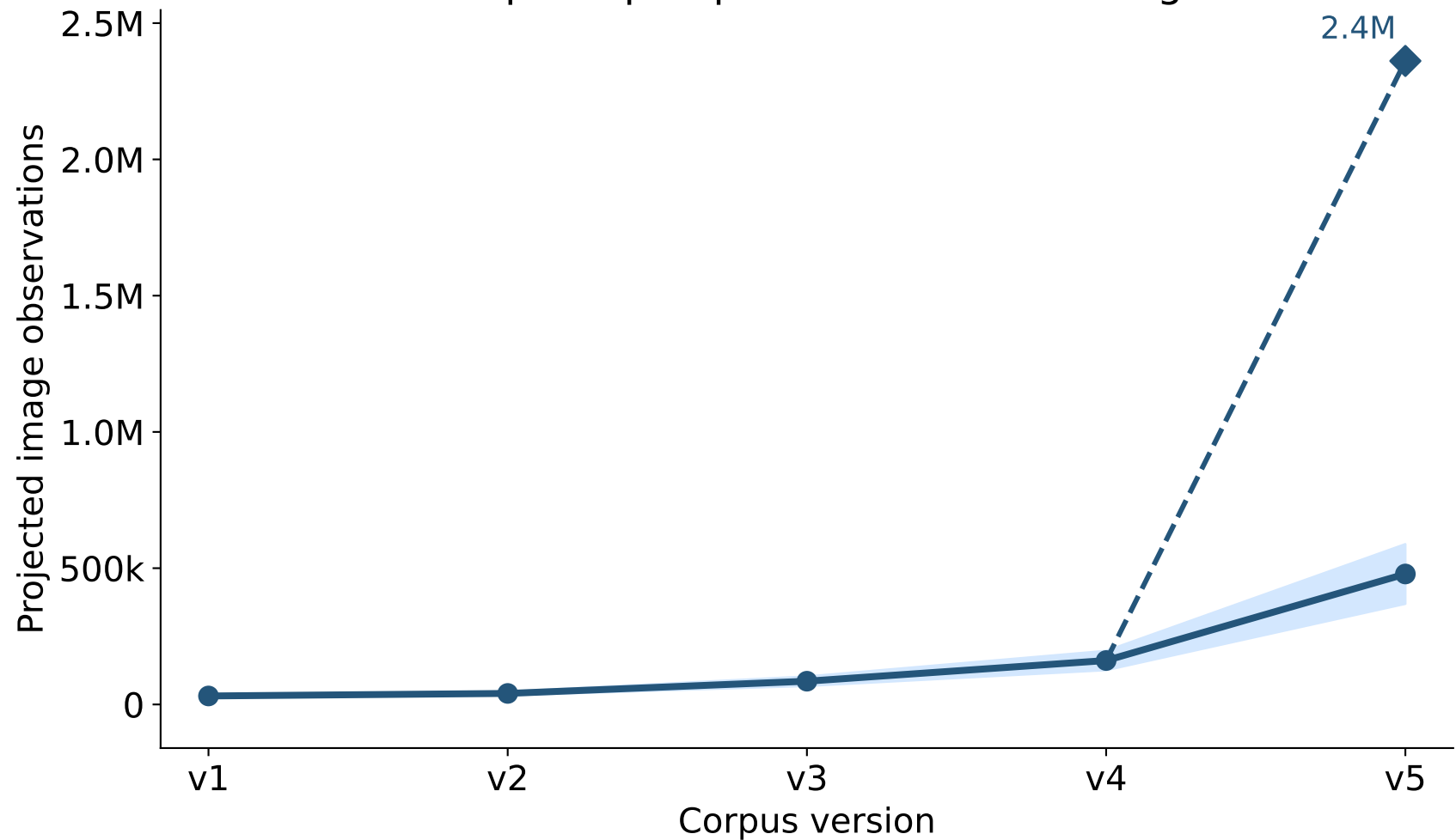
Cumulative MorphSeq corpus: effect of retaining five z-slices
