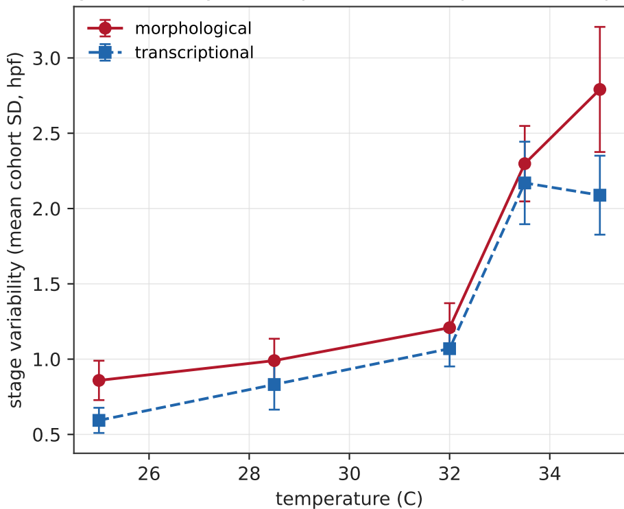
Stage variability vs temperature · morph + transcription
