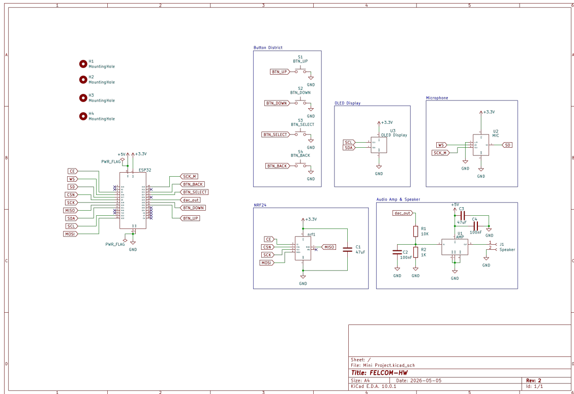
Figure 3: Full hardware schematic of a FELCOM unit (ESP32, nRF24L01+, INMP441, audio amplifier, OLED and controls)
