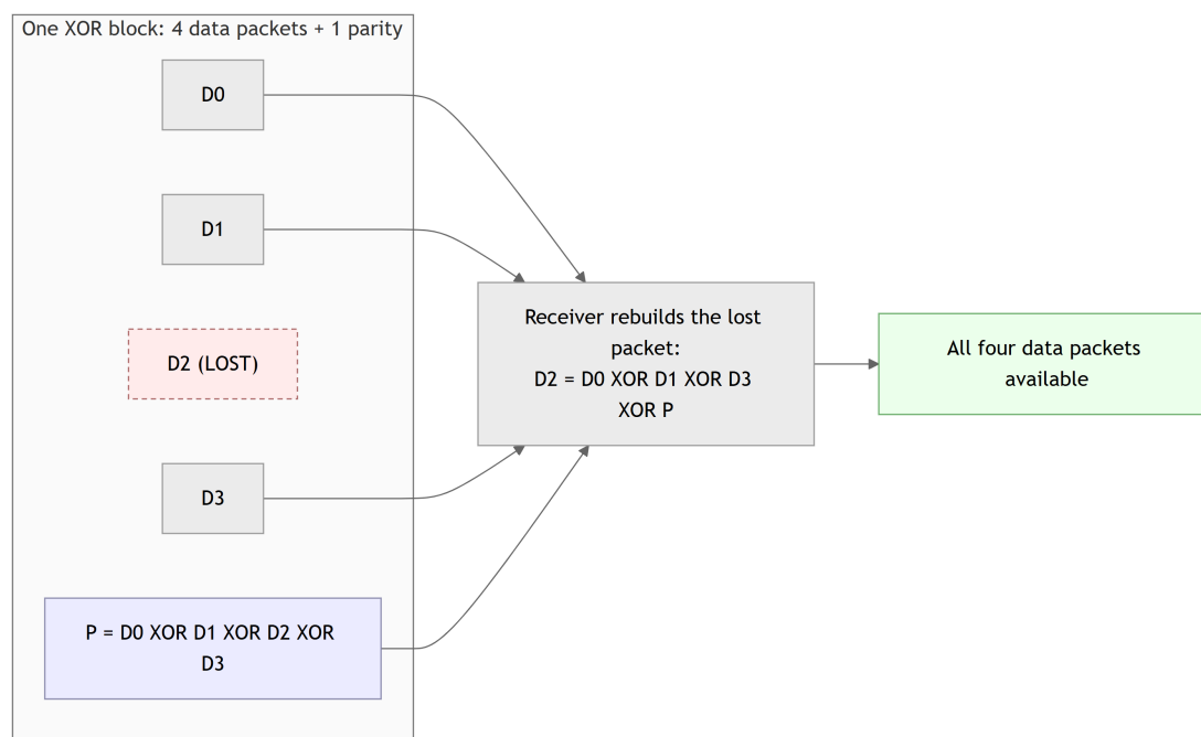
Figure 7: XOR block forward error correction: one lost packet per block of four is reconstructed from the parity packet.
