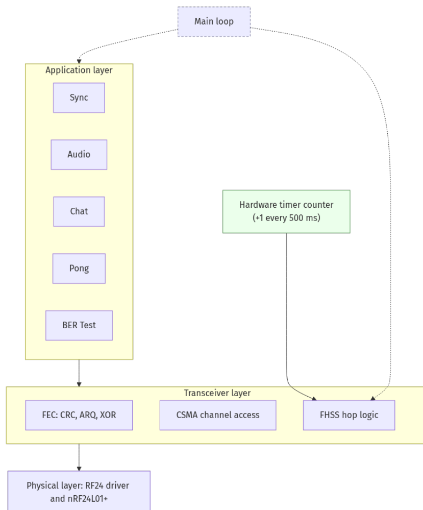
Figure 5: Layered firmware architecture and the non-blocking main loop.
