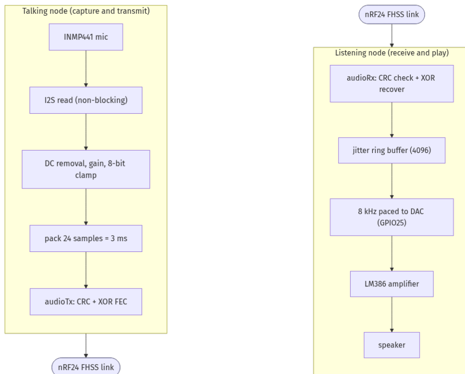
Figure 9: The non-blocking real-time audio pipeline, from microphone to speaker.
