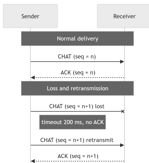
Figure 8: ARQ exchange for reliable chat delivery, including retransmission on timeout.
