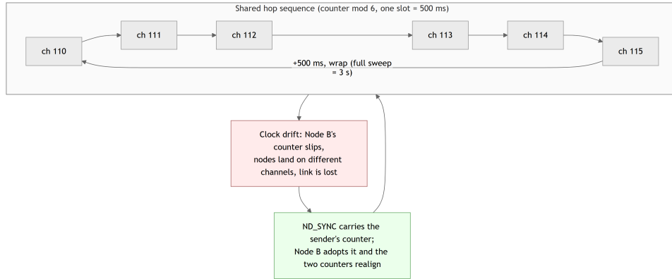
Figure 5: Timer-driven hopping schedule across the six channels and re-alignment via an ND_SYNC packet.
