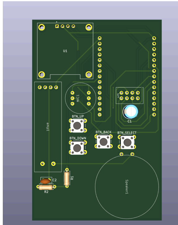
Figure 3: The custom-designed FELCOM PCB layout.
