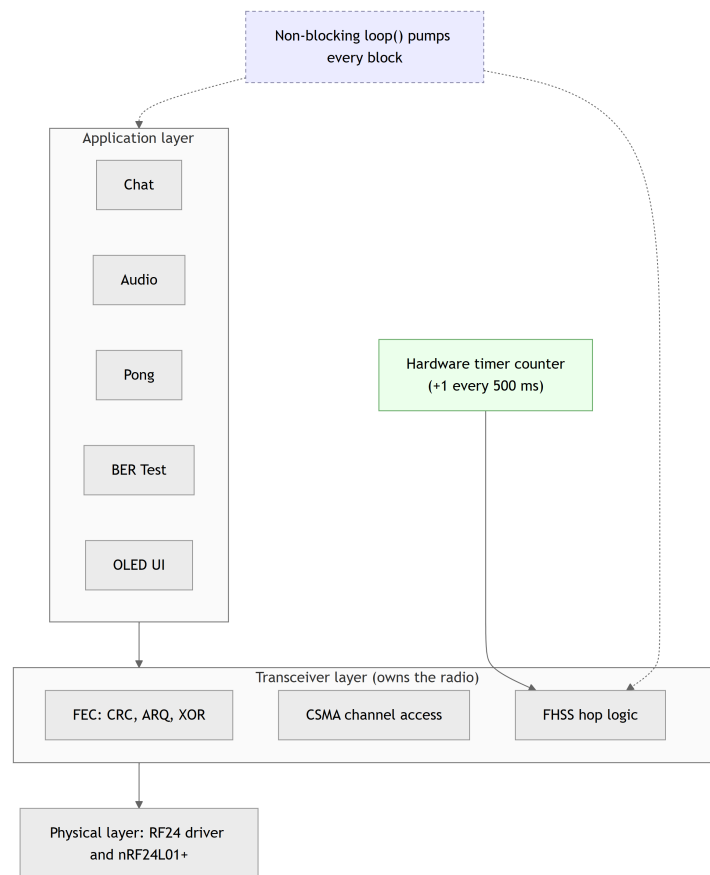
Figure 4: Layered firmware architecture and the non-blocking main loop.
