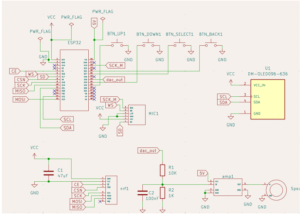
Figure 2: Full hardware schematic of a FELCOM unit (ESP32, nRF24L01+, INMP441, audio amplifier, OLED and controls).
