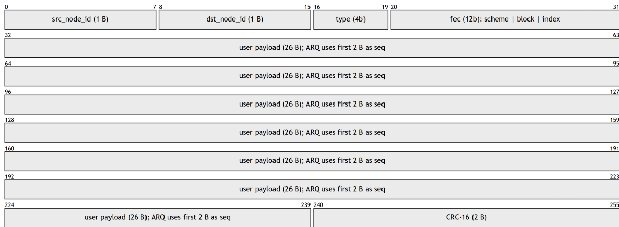
FELCOM 32-byte on-air frame
