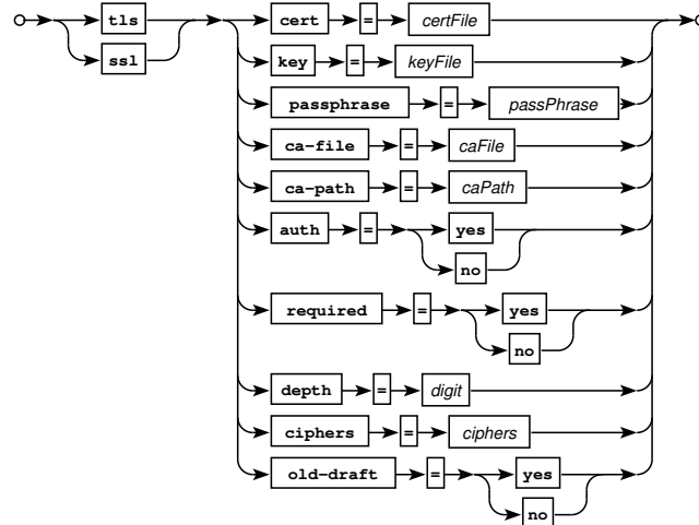
Railroad diagram: TLSExpr
