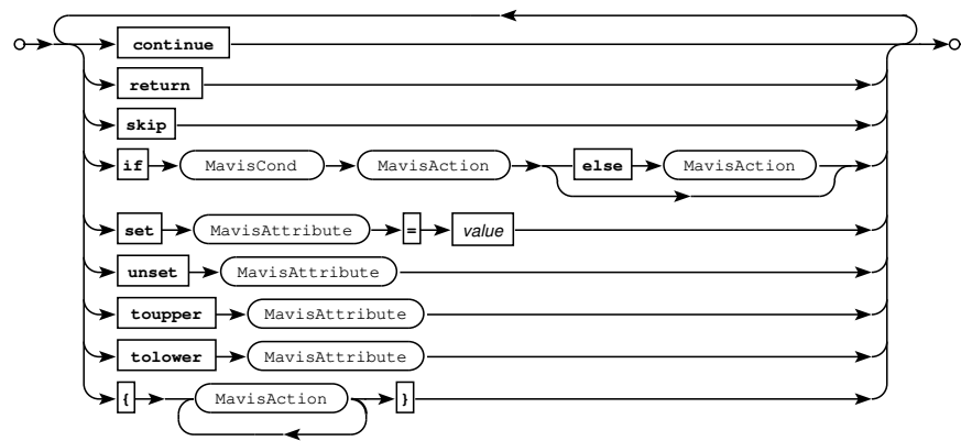
Railroad diagram: MavisAction
