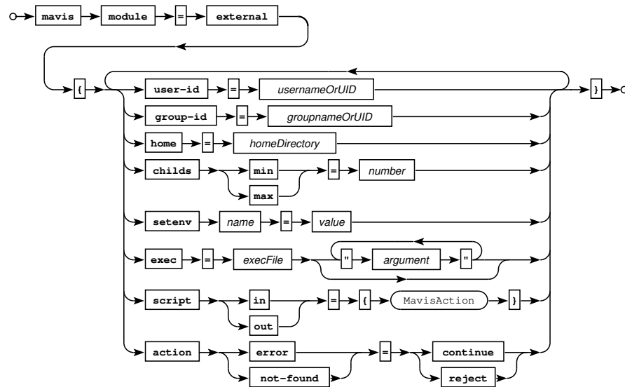
Railroad diagram: ExternalConf
