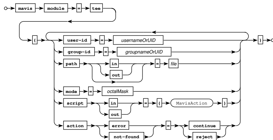
Railroad diagram: TeeConf
