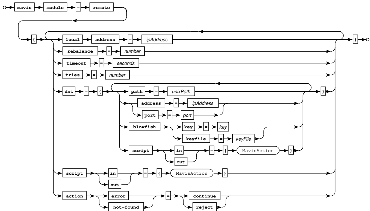
Railroad diagram: RemoteConf
