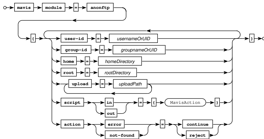
Railroad diagram: AnonftpConf
