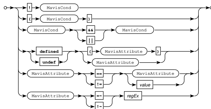
Railroad diagram: MavisCond
