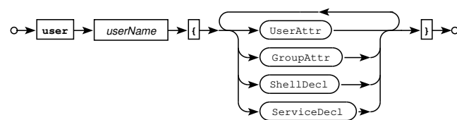
Railroad diagram: UserDecl
