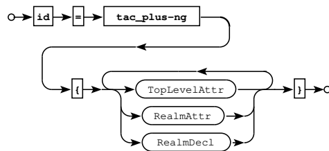
Railroad diagram: TacPlusConfig
