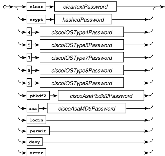
Railroad diagram: PasswordExprHash
