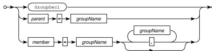
Railroad diagram: GroupAttr
