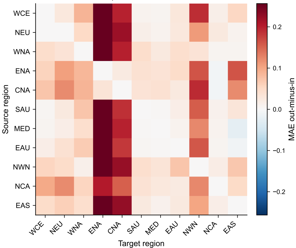
Graph WaveNet transfer
