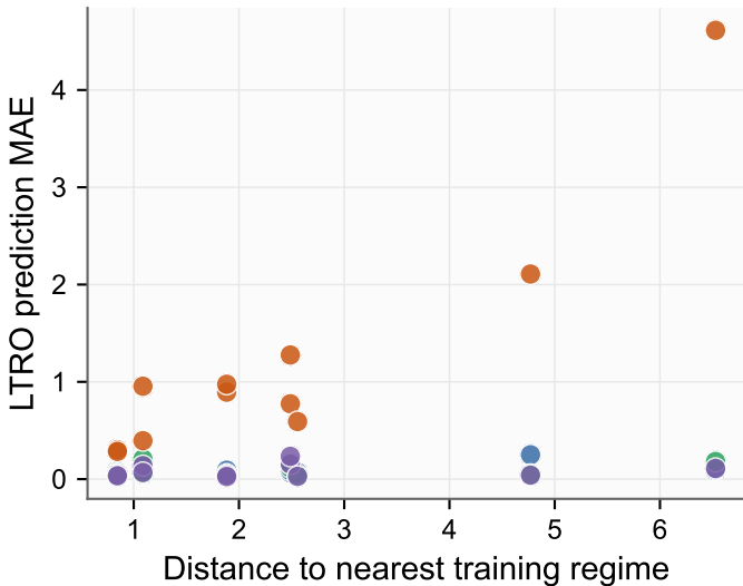
Prediction error
