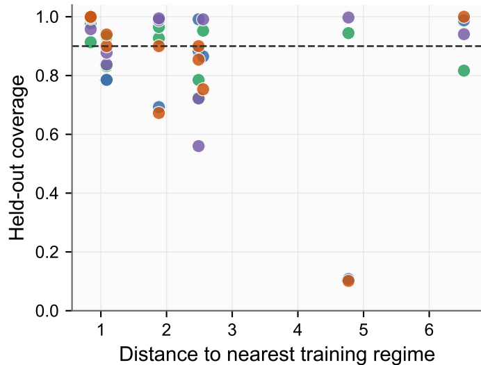
Conformal coverage
