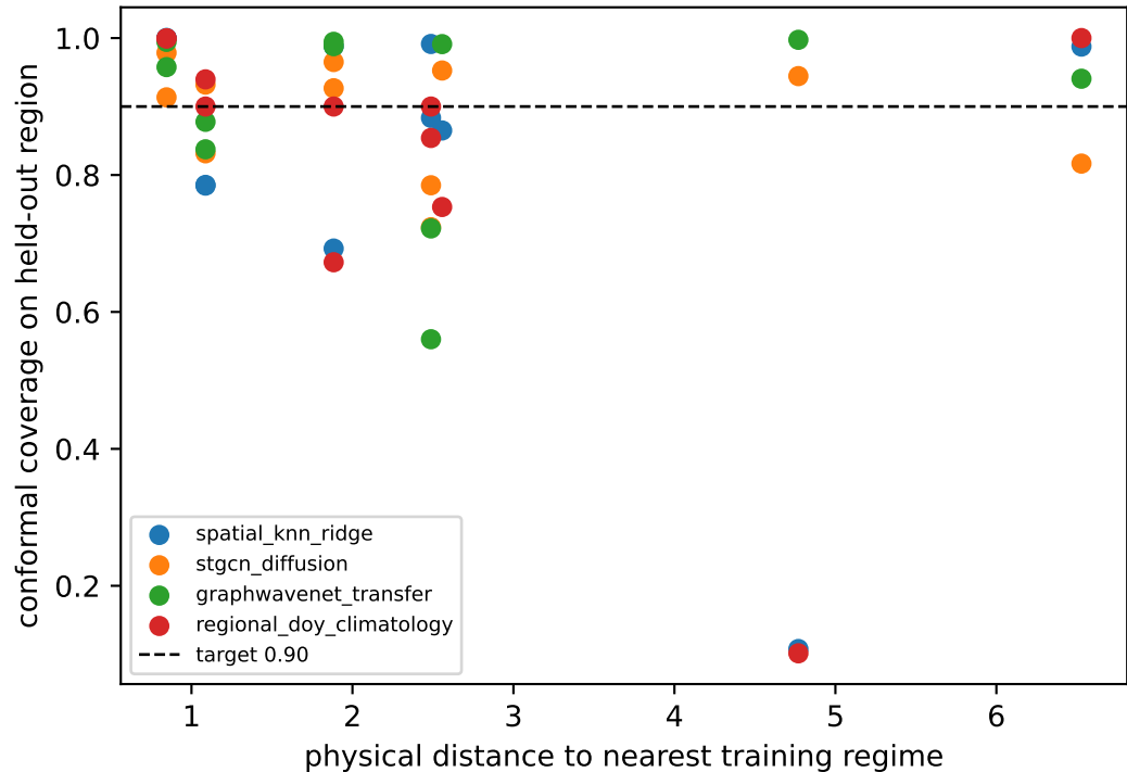
Regime-conditional conformal coverage
